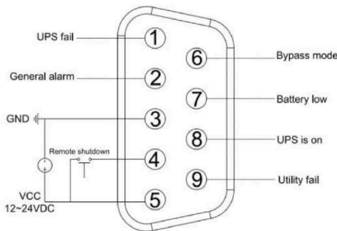
RS-232 Serial Port (DB-9 Connector)
